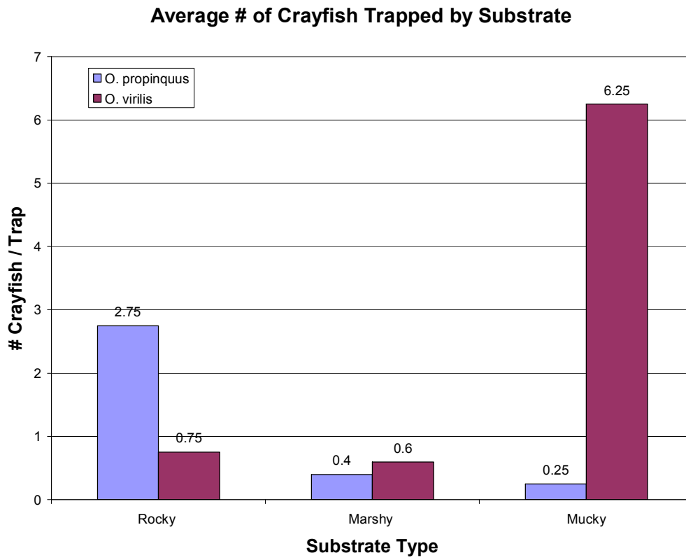
Figure 3: Average number of species caught per trap at each substrate type.
